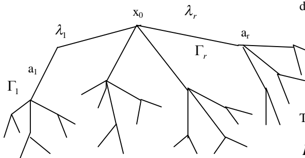
Figure1. Truncating \Gamma
