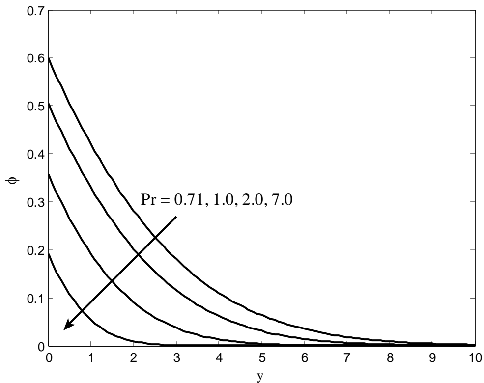
Figure 4: Temperature profiles for different values of Pr
