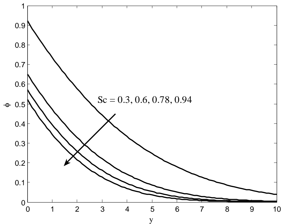
Figure 6: Concentration profiles for different values of Sc
