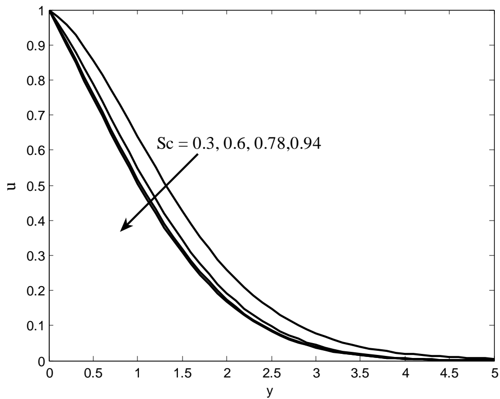
Figure 5: Velocity profiles for different values of Sc
