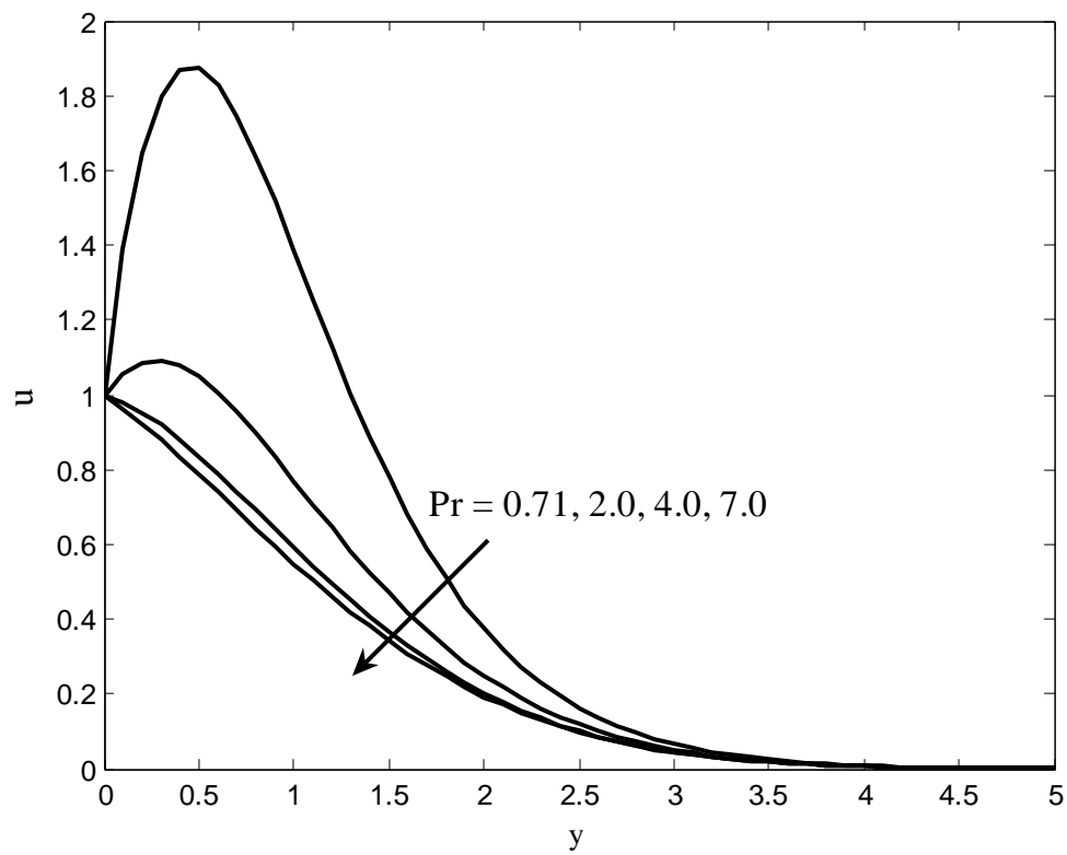
Figure 3: Velocity profiles for different values of Pr
